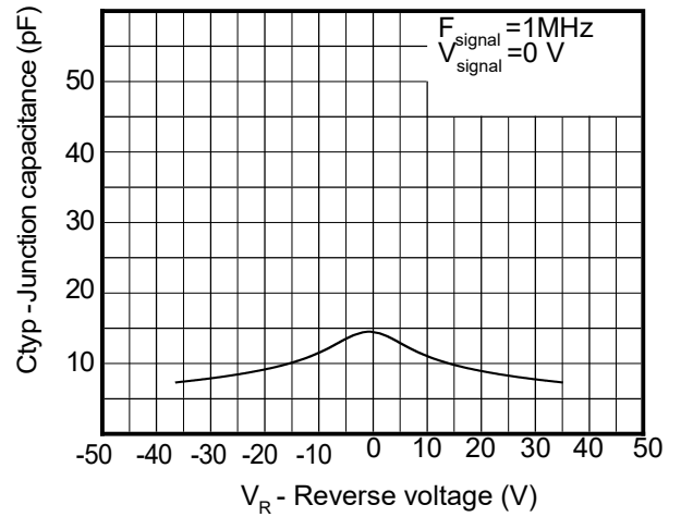
Capacitance vs. Revers voltage
