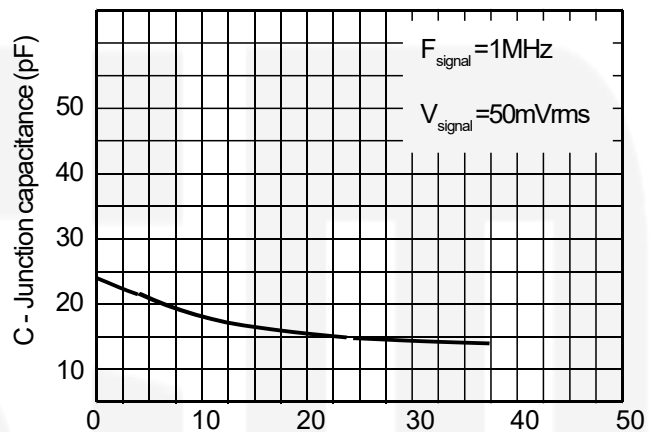
Capacitance vs. Reverses voltage
